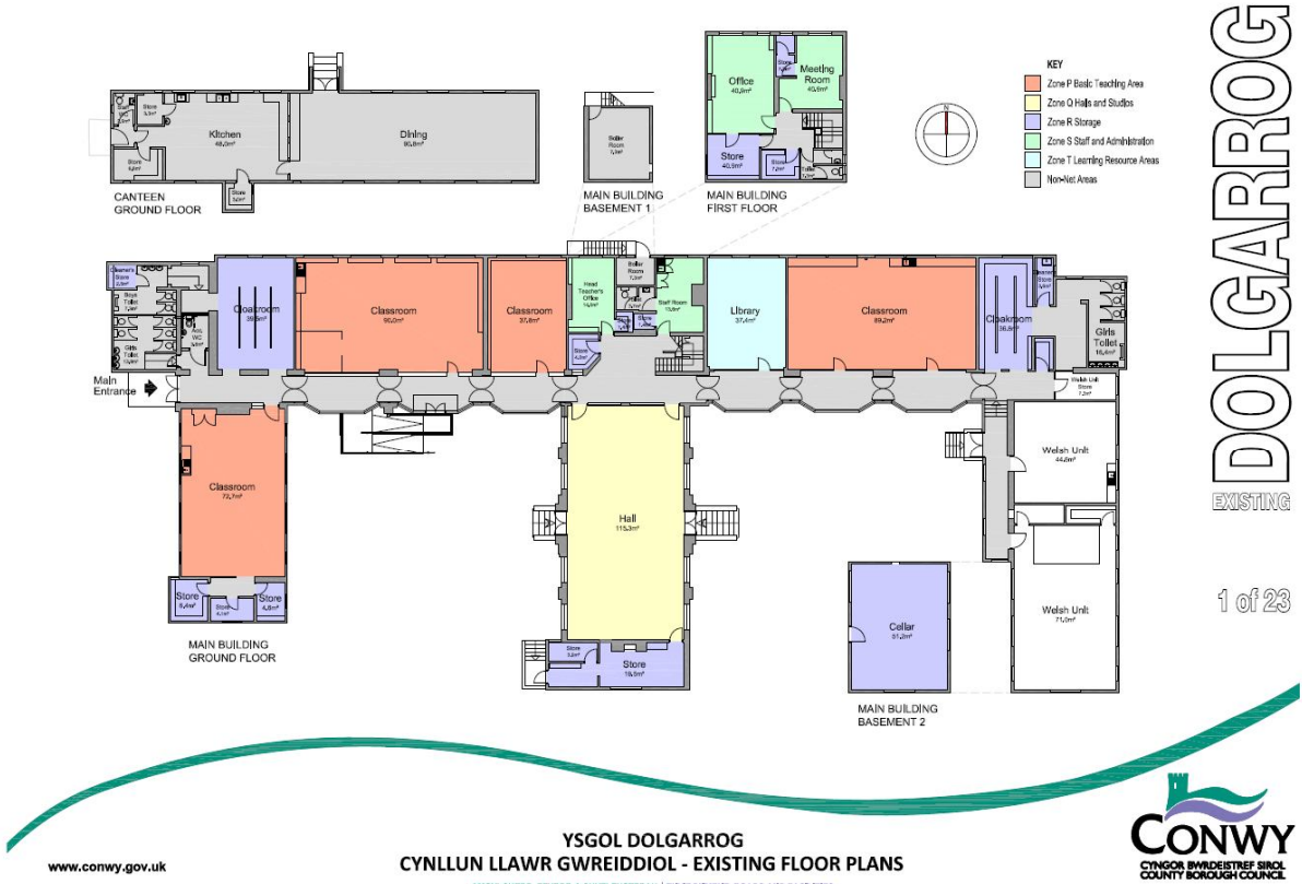
Plan of buildings
