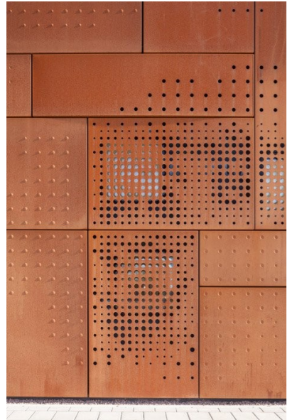
Sgrin law dur Cor-Ten Cor-Ten steel rainscreen cladding
