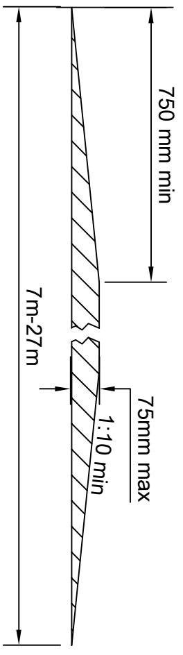
Trawslun of fwrdd arafu Speed table cross section
