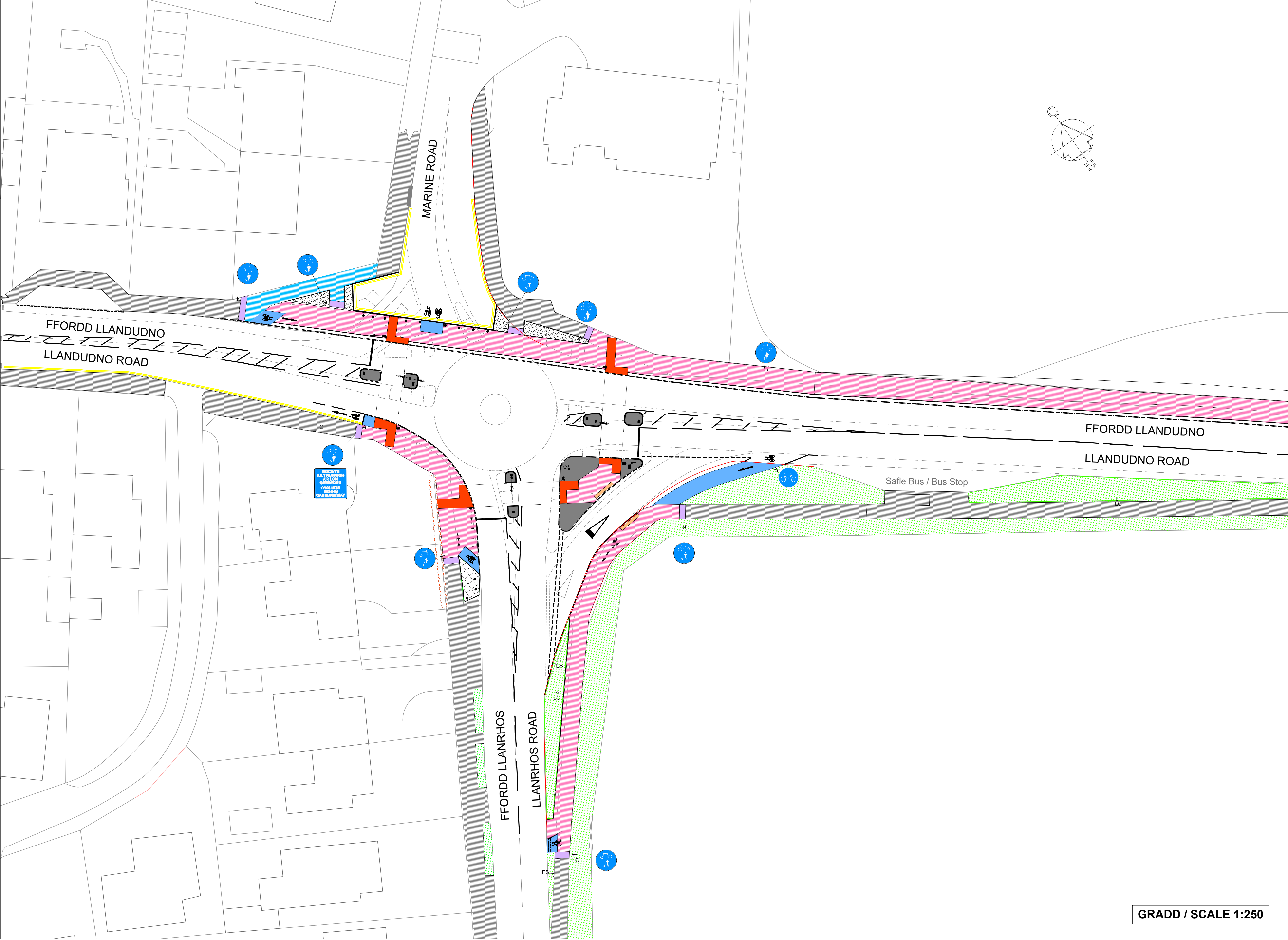
CYNLLUN 1 - CYFFORDD TOLL BAR DEWIS 1 DRAWING 1 - TOLL BAR JUNCTION OPTION 1
