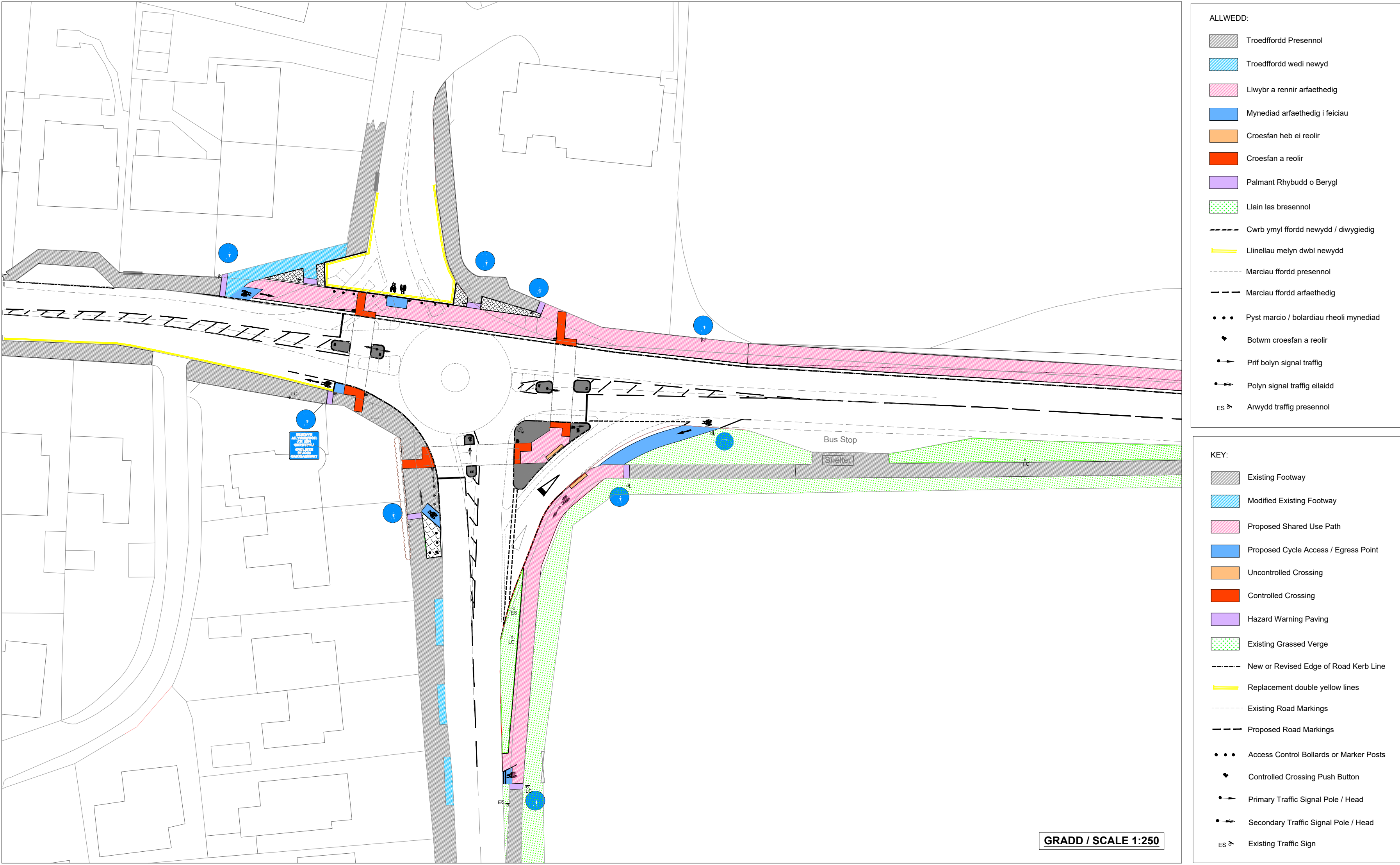
CYNLLUN 1 - CYFORDD TOLL BAR DRAWING 1 - TOLL BAR JUNCTION
