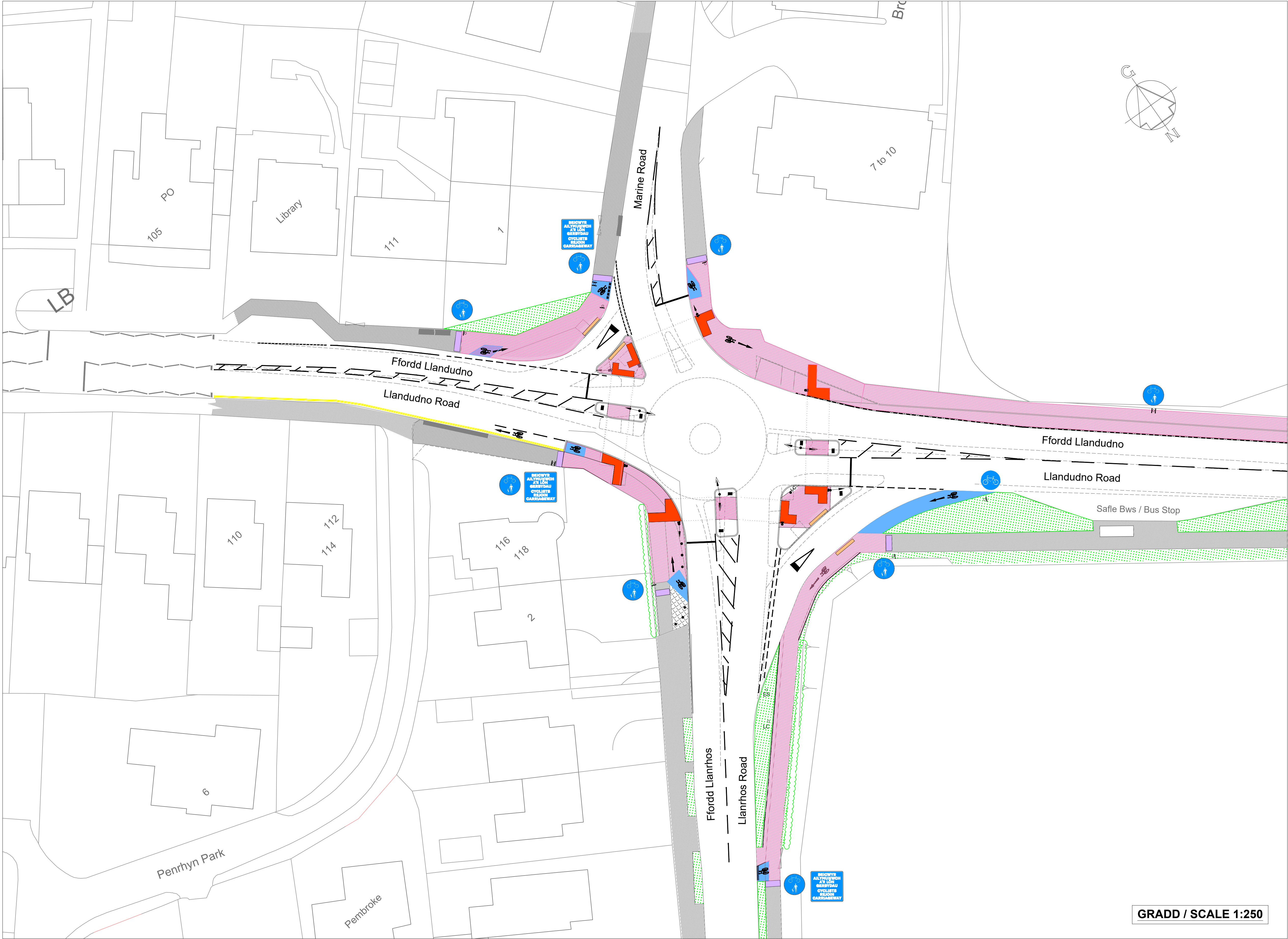
CYNLLUN 1B - CYFFORDD TOLL BAR DEWIS 2 DRAWING 1B - TOLL BAR JUNCTION OPTION 2
