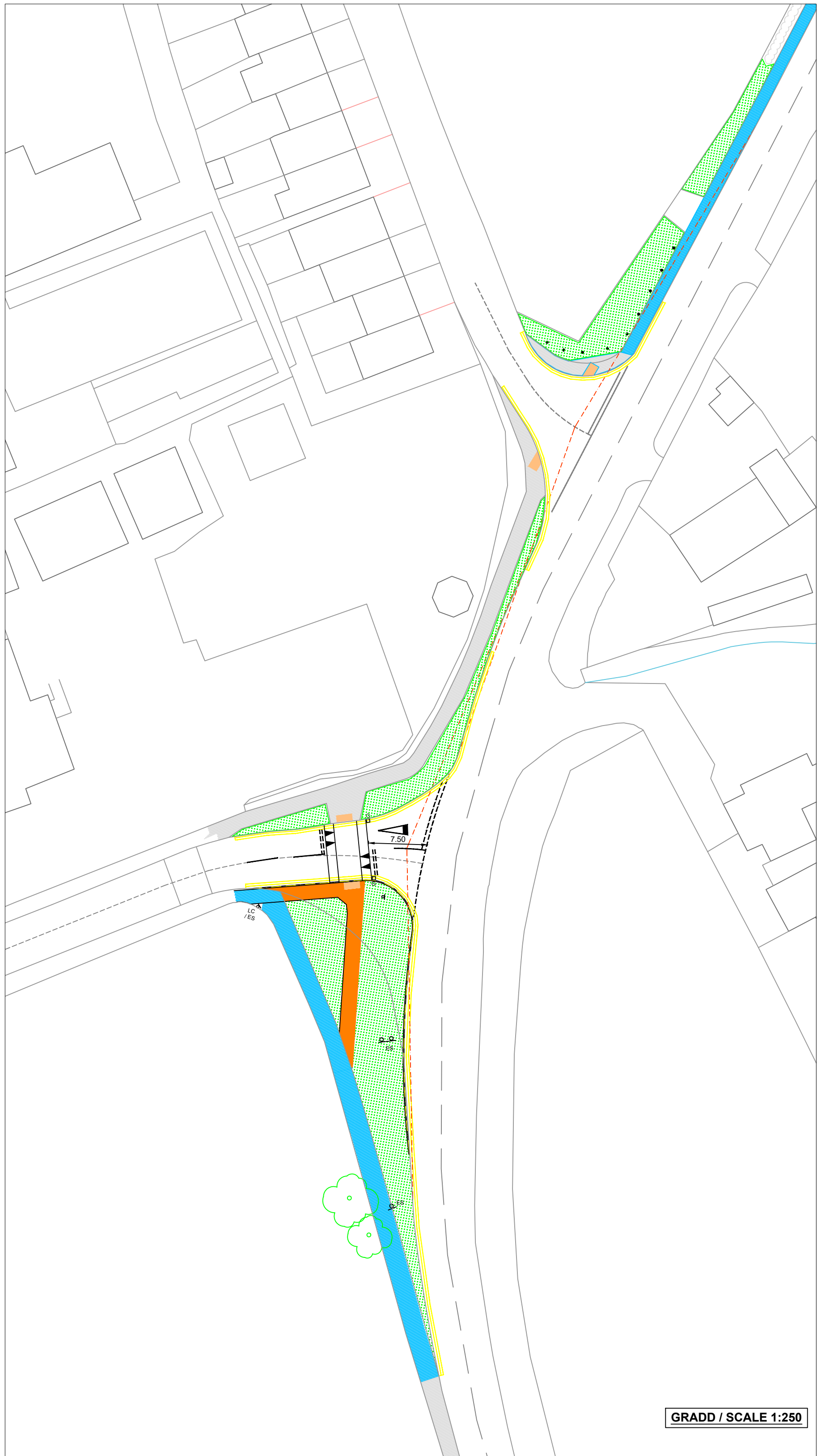
CYNLLUN 4 - LLANRHOS ROAD / LON DERWEN DRAWING 4 - LLANRHOS ROAD / DERWEN LANE
