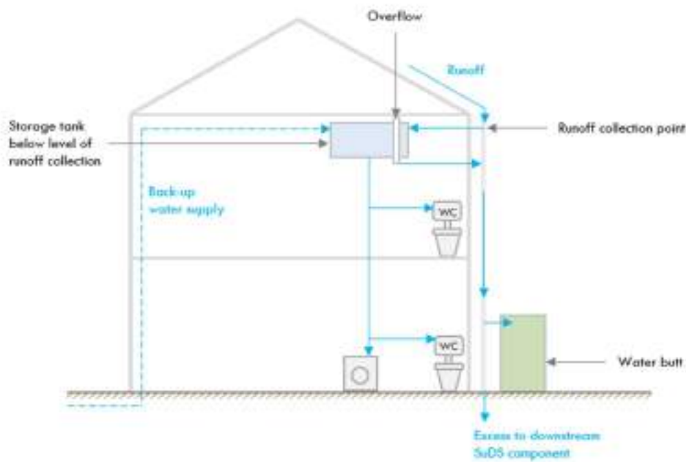
Gravity RWH system concept
