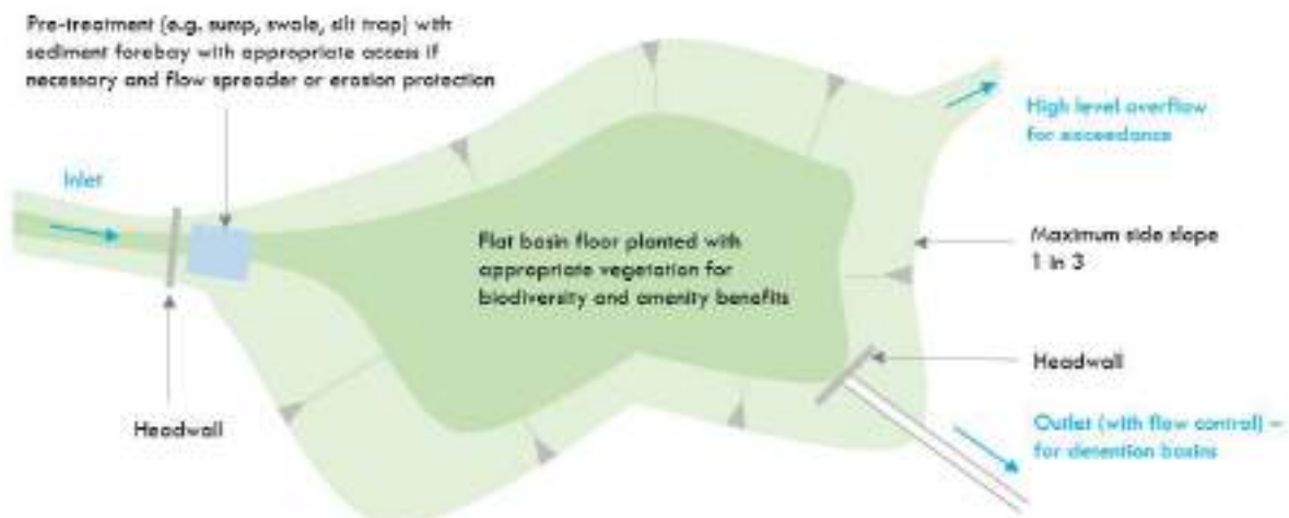
Basin plan
