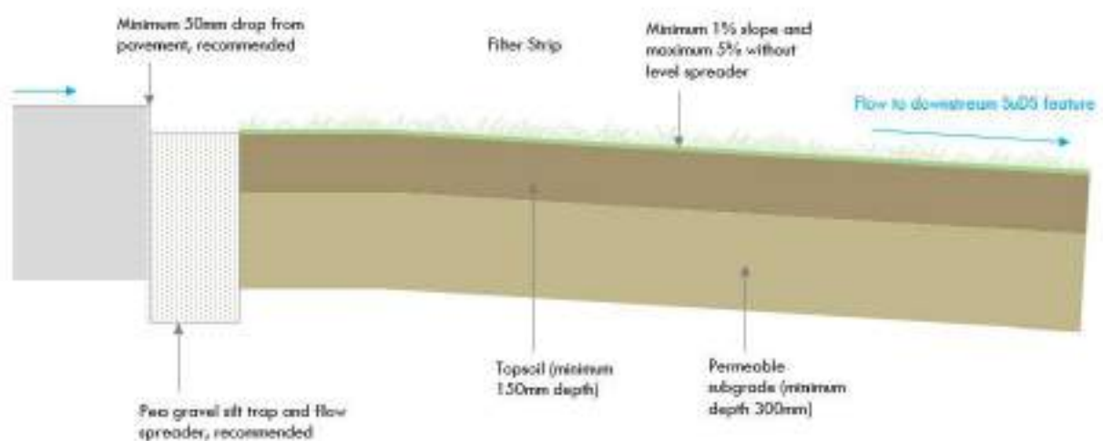
Filter strip
