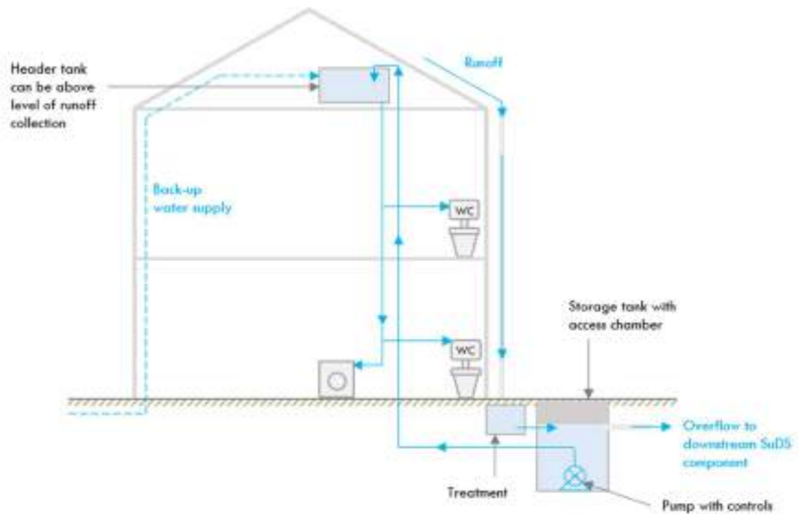
Pumped RWH system concept
