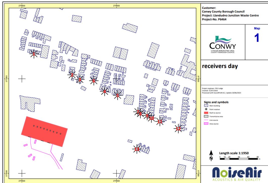
Figure 9: Illustration of the 3D sound model selected facades receptors.
