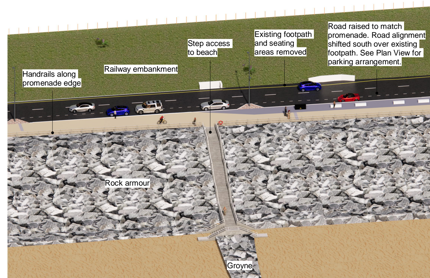
7 3D VIEW - BEACH ACCESS STEPS
