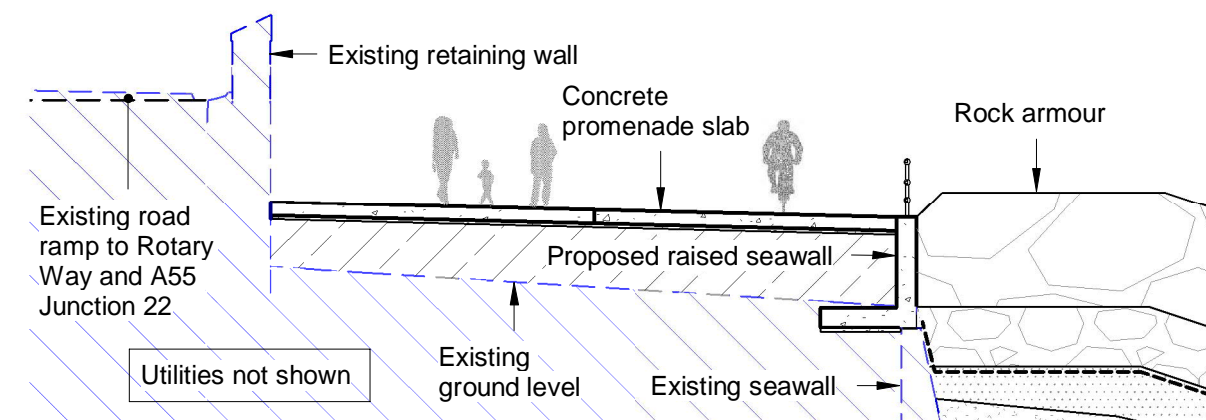
6 SECTION VIEW - TYPICAL ARRANGEMENT (CENTRAL) 1 : 150
